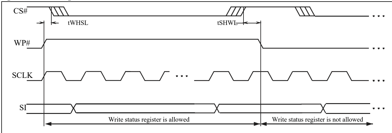
Figure 4-7 WP Timing
